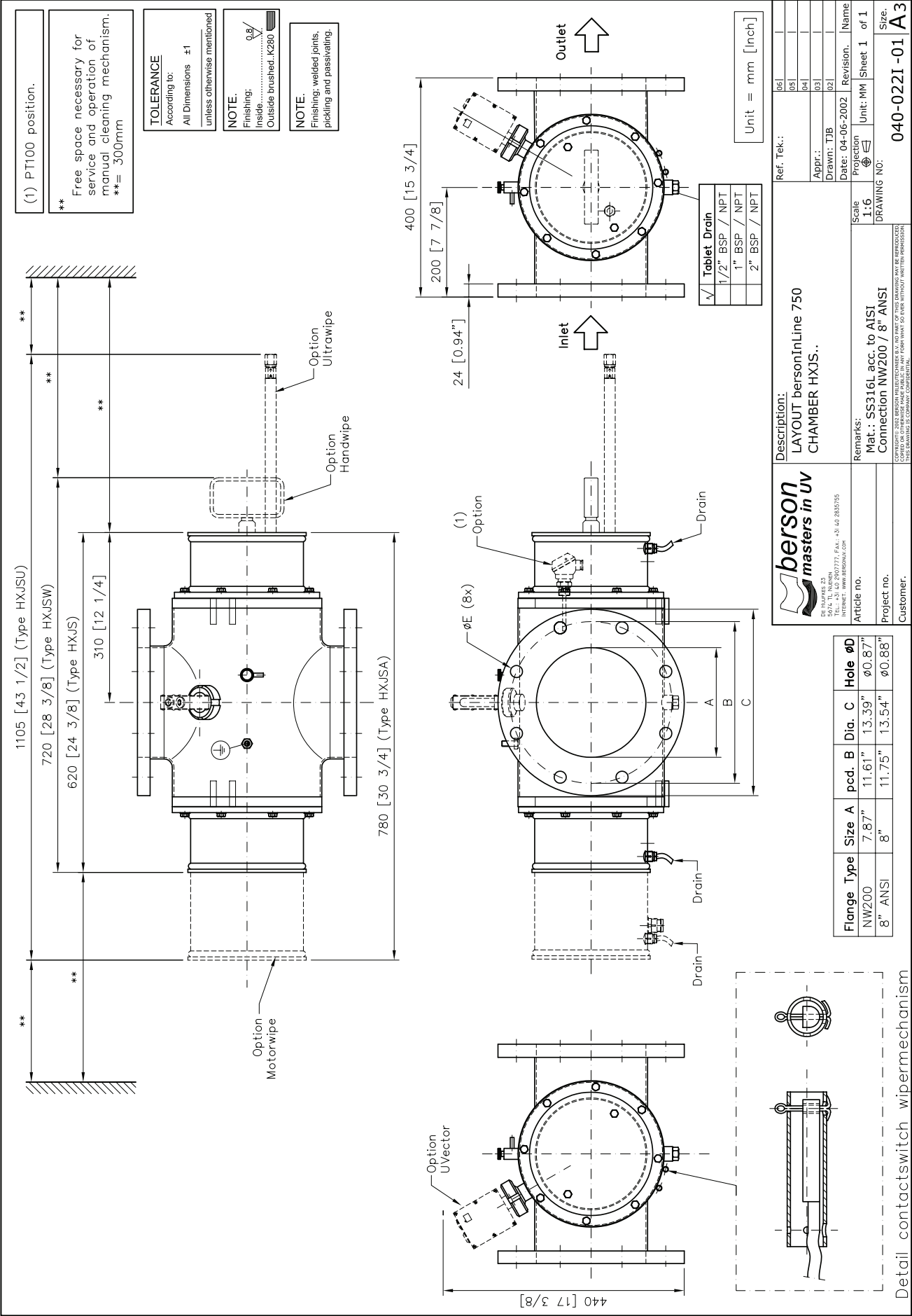
Layout drawing bersonInLine 750 ST
