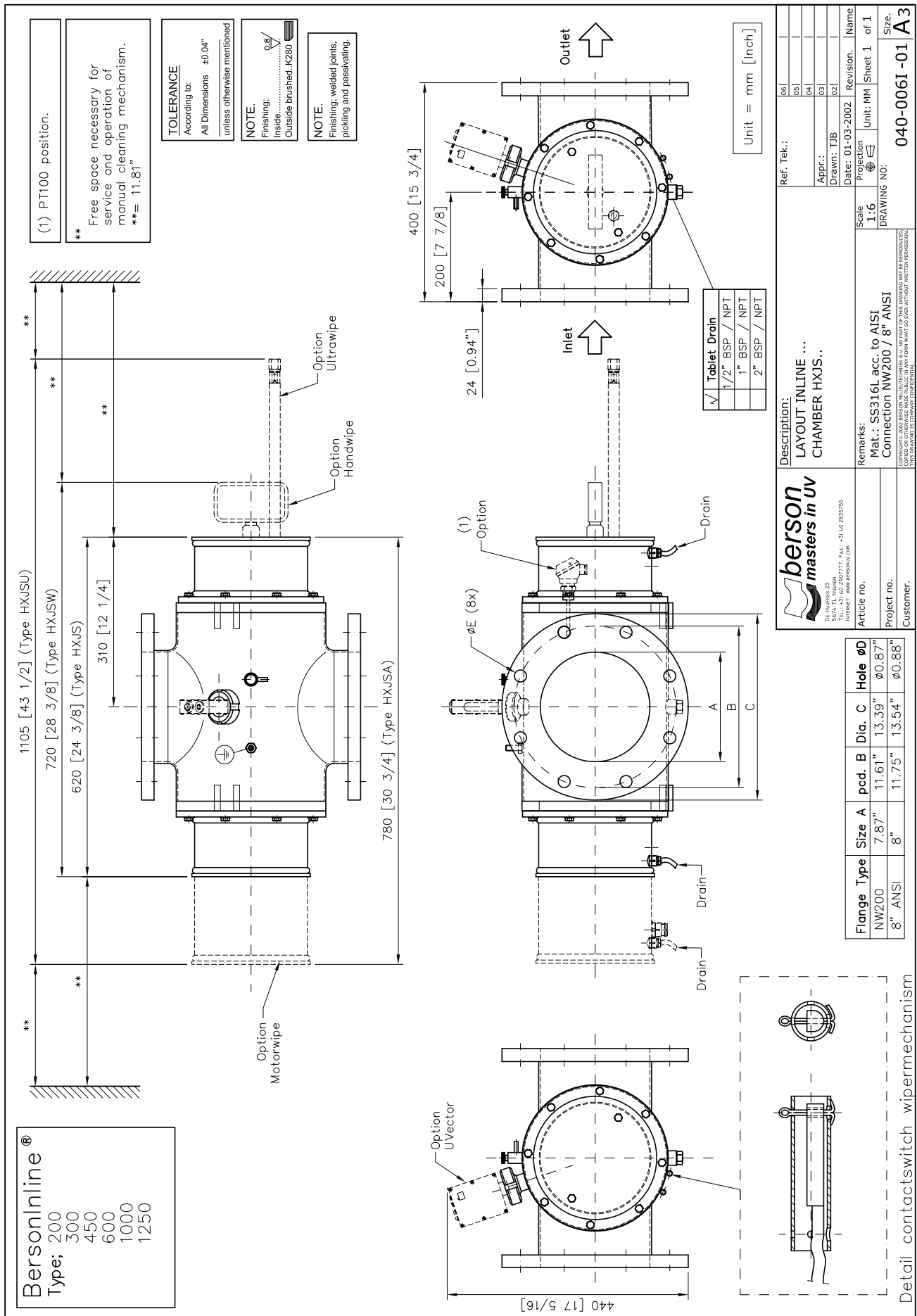
Layout drawing bersonInLine 200 ST
